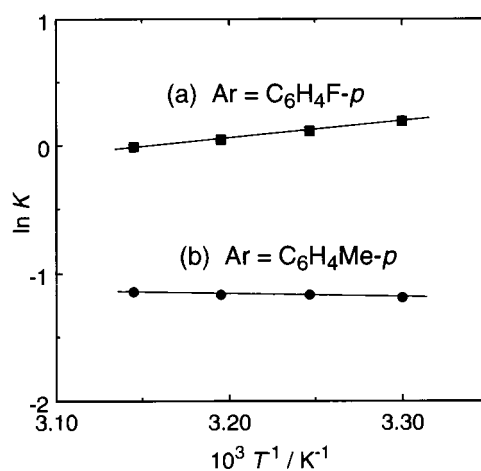
Fig. 4 Van't Hoff plots of the reactions (a) \mathbf{2a} + \text{CH}_2=\text{CCH}_2\text{CHC}_6\text{H}_4\text{F-}p \longrightarrow \mathbf{2b} + \text{CH}_2=\text{CCH}_2\text{CHC}_6\text{H}_5 and (b) \mathbf{2a} + \text{CH}_2=\text{CCH}_2\text{CHC}_6\text{H}_4\text{Me-}p \longrightarrow \mathbf{2c} + \text{CH}_2=\text{CCH}_2\text{CHC}_6\text{H}_5 .
