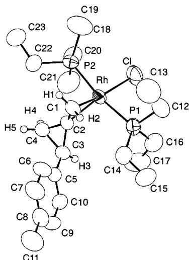
Fig. 2 An ORTEP drawing of [\text{RhCl}(\text{CH}_2=\text{CCH}_2\text{CHC}_6\text{H}_4\text{Me-}p\text{)}(\text{PEt}_3)_2] 3c with 50% thermal ellipsoidal plotting. Hydrogen atoms except for those in vinyl and cyclopropyl groups were omitted for simplicity. Selected bond distances (Å) and angles ( ^\circ ): Rh–Cl 2.373(2), Rh–P1 2.323(2), Rh–P2 2.319(2), Rh–C1 2.105(7), Rh–C2 2.047(7), C1–C2 1.405(9), C2–C3 1.497(9), C2–C4 1.465(10) and C3–C4 1.528(10); Cl–Rh–P1 86.45(8), Cl–Rh–P2 86.31(8), P1–Rh–P2 171.18(7), C1–Rh–C2 39.5(3), Rh–C1–C2 68.0(4), Rh–C2–C1 72.4(4), C1–C2–C3 136.8(7), C1–C2–C4 136.5(7), C2–C3–C4 57.9(5), C2–C4–C3 60.0(5), C3–C2–C4 62.1(5), H1–C1–H2 107, C2–C1–H1 119 and C2–C1–H2 120.
