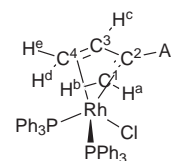
Chart 1 Numbering scheme of complexes 1a–1d .
